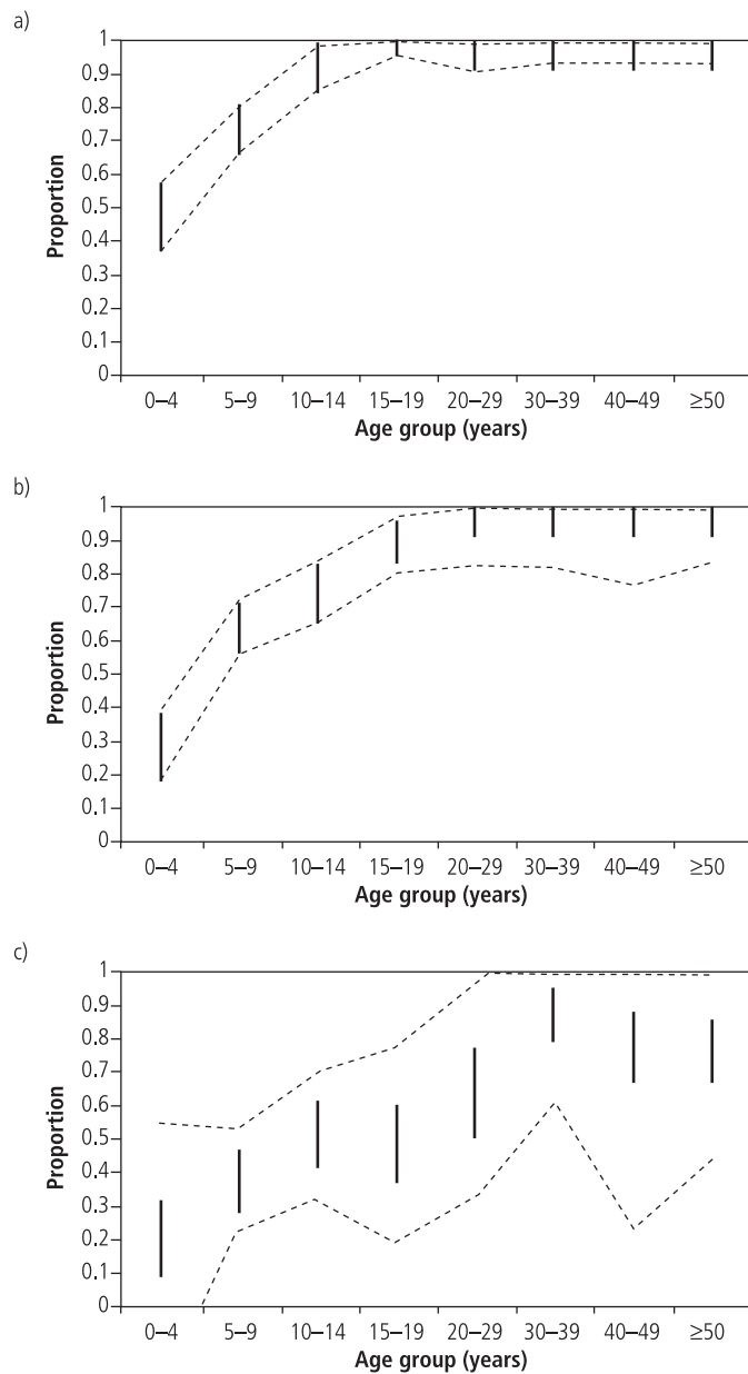
Fig. 2. Upper and lower 95% confidence limits for predicted "true" antibody prevalence, p_T , estimated from oral fluid prevalence, p_o (dotted lines), using eq. (1) (see Methods), compared with 95% confidence limits for seroprevalence (vertical lines), for a) measles, b) rubella, and c) hepatitis B core antigens in Butajira District, southern Ethiopia, 1997
