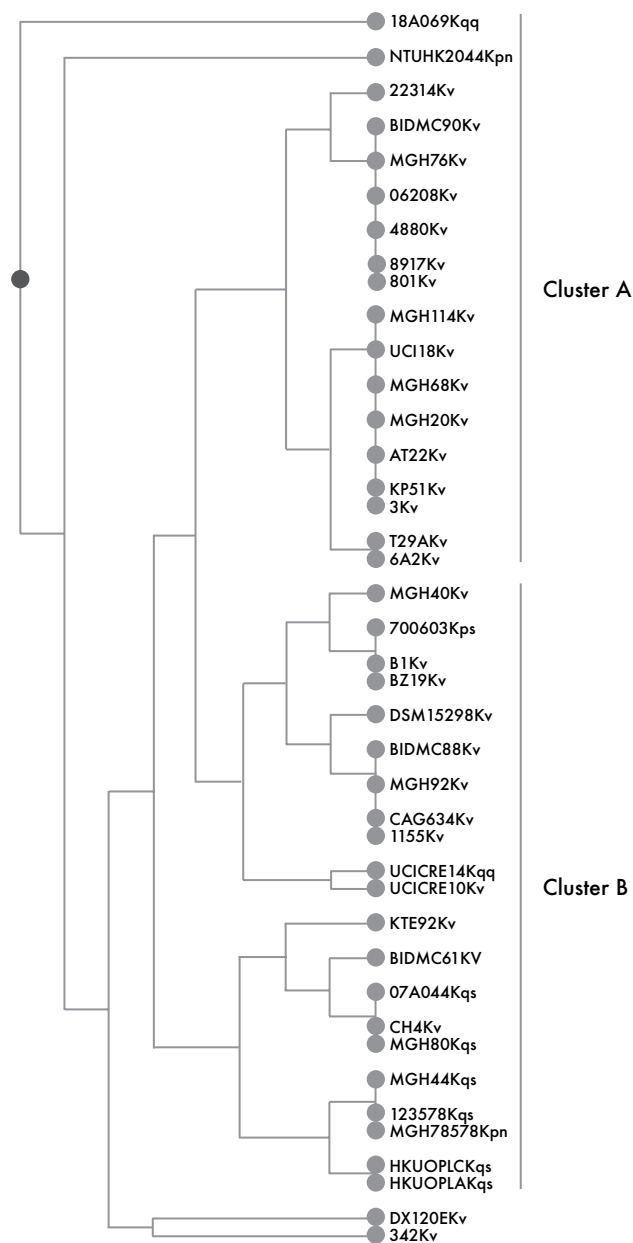
FIGURE 2. JACQUARD INDEX OF THE PLANT-DETERMINANT PROTEINS OF THE K. VARIICOLA (Kv), K. QUASIPNEUMONIAE (Kq) AND K. PNEUMONIAE (Kpn) GENOMES
